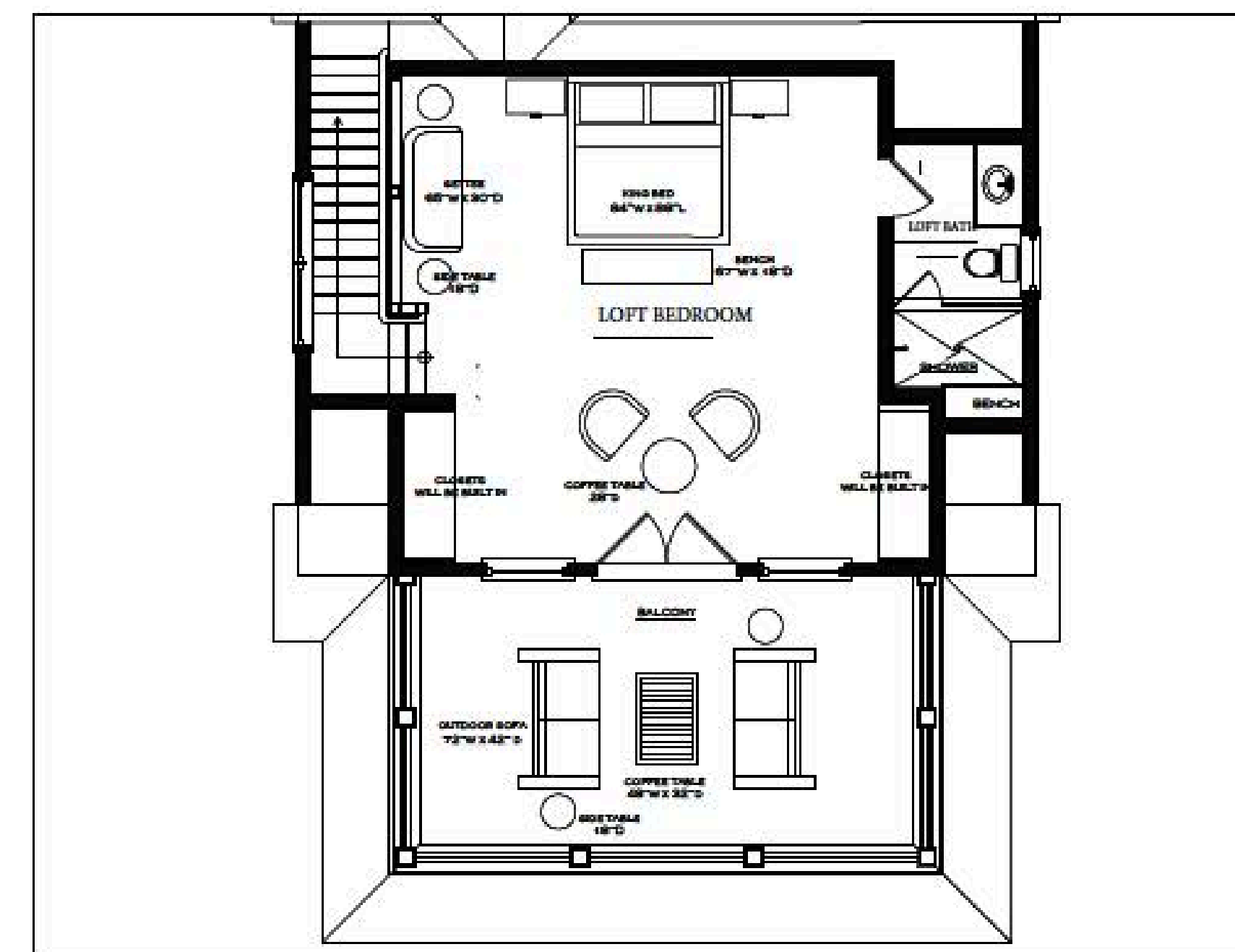
2 SECOND FLR - GUEST ROOM SUITE SCALE: 3/16" = 1'-0"
